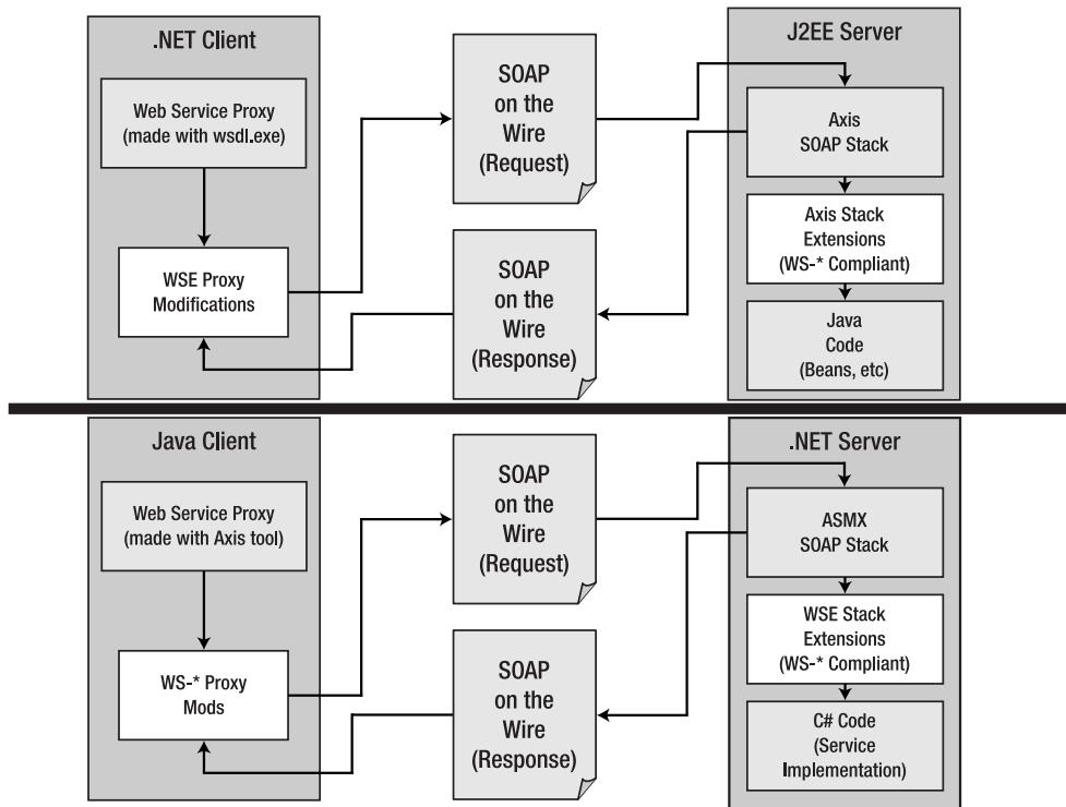
Figure 6-22. WS-* Interoperability
