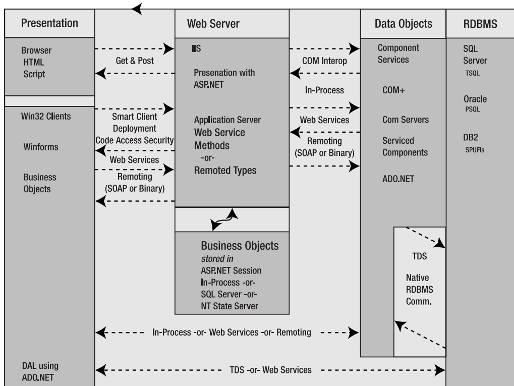
Figure 1-1. .NET solutions
