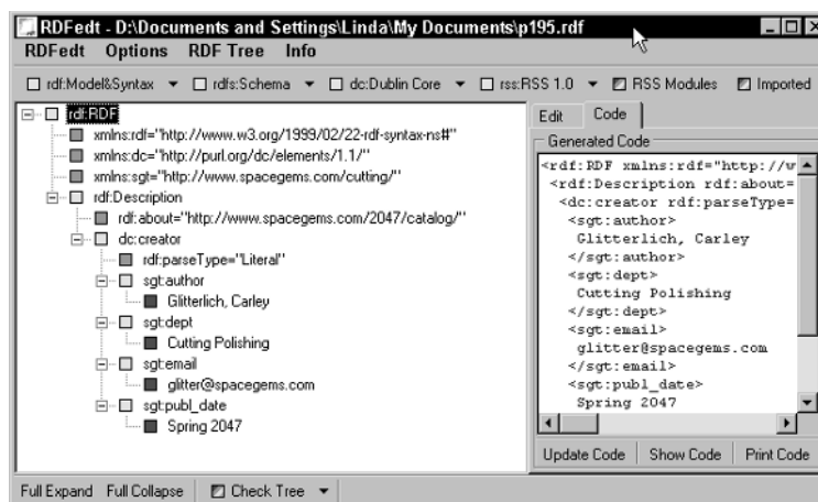
Figure 13.6 RDFedit file with all elements and attributes added.
