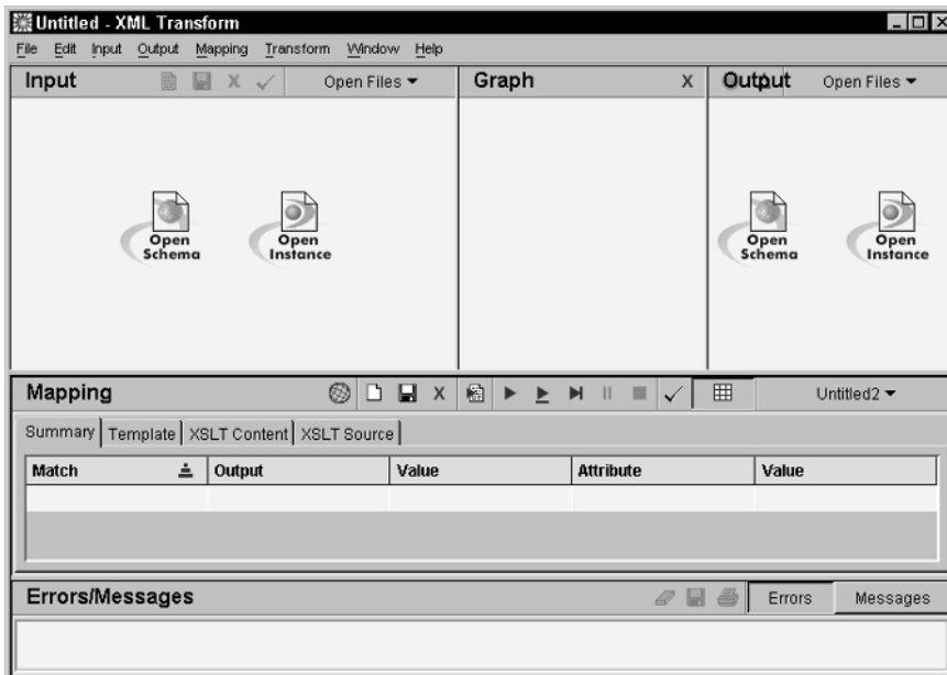
Figure 9.7 XMLTransform workspace.
