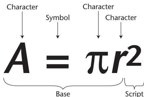
Figure 16.4 Dissected equation.
