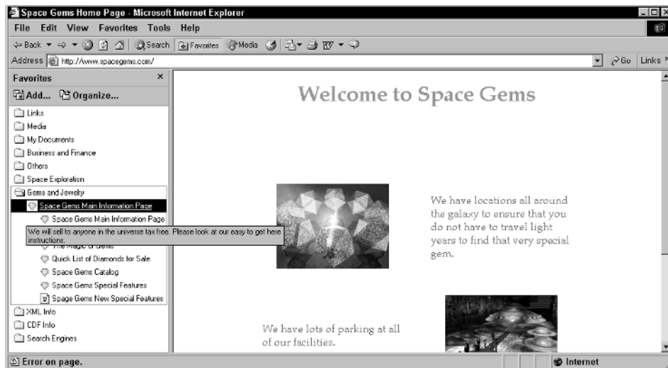
Figure 14.11 ToolTip example.
