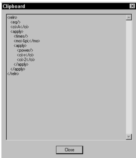
Figure 16.21 Content markup source code, as depicted by EzMath editor.
