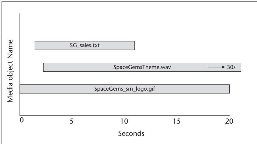
Figure 12.9 The <par> element.
