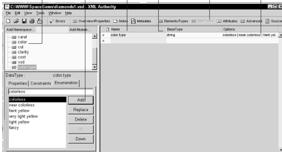
Figure 5.12 Creating the color.type data type for the <color> element.
