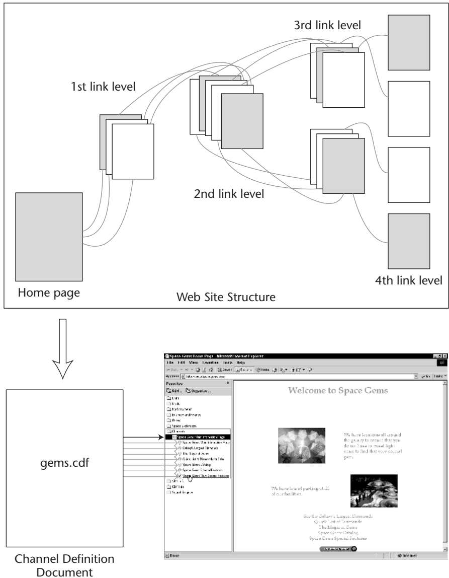
Figure 14.8 Simplified channel development schematic.
