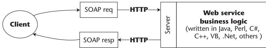
Figure 15.2 SOAP request/response process.
