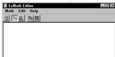
Figure 16.18 EzMath Editor.
