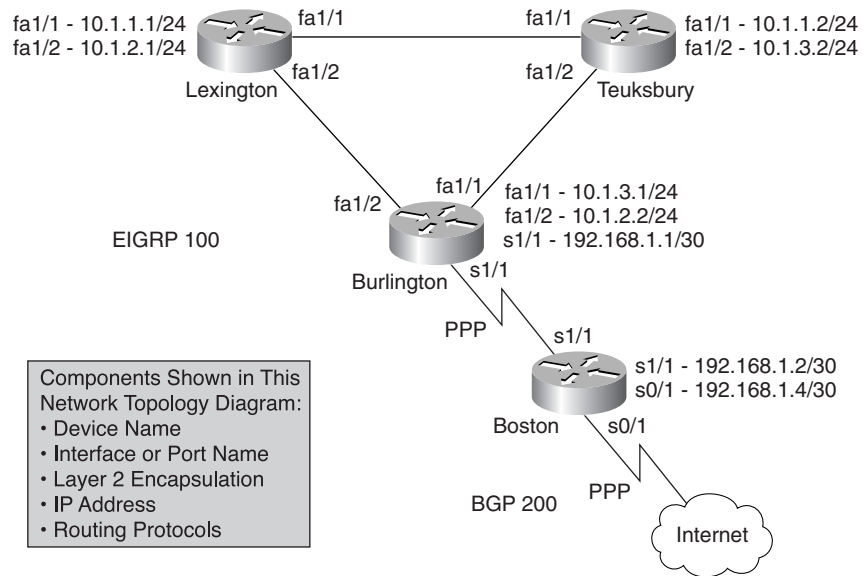
Figure 1-1 Network Topology Diagram
