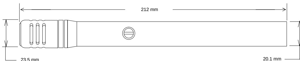
OVERALL DIMENSIONS FIGURE 3
