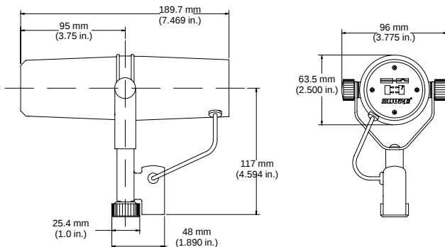
OVERALL DIMENSIONS FIGURE 3
