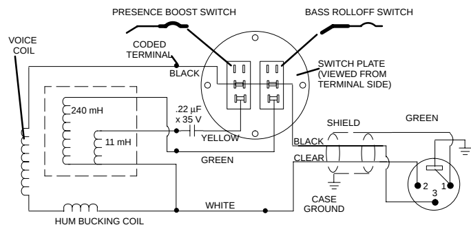
INTERNAL CONNECTIONS FIGURE 4
