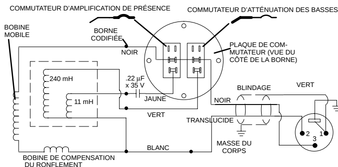
BRANCHEMENTS INTERNES FIGURE 4
