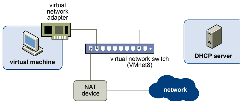
Figure 12-2. NAT Configuration
